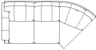
7029-LAF Birchfield Left Arm Facing Sofa w/ Built-In Half Round Overall: H40 W89 D41 Inside: W67 D22 Seat: H21 Arm: H25
